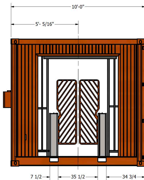
BACK VIEW
