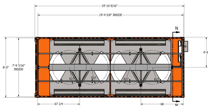
SECTION B-B 2025-127-000, ROOF PANELS REMOVED FOR CLARITY
